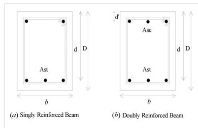
Figure 1. Sectional details of rectangular beams
