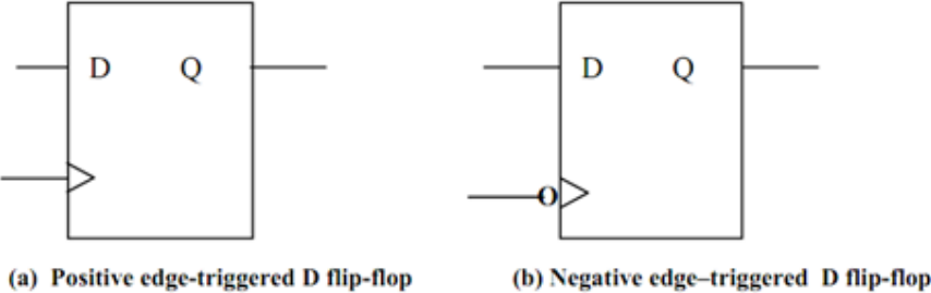
Figure : Edge triggered D flip- flops
