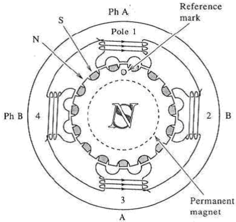
Cross-section of a two-phase hybrid motor.
