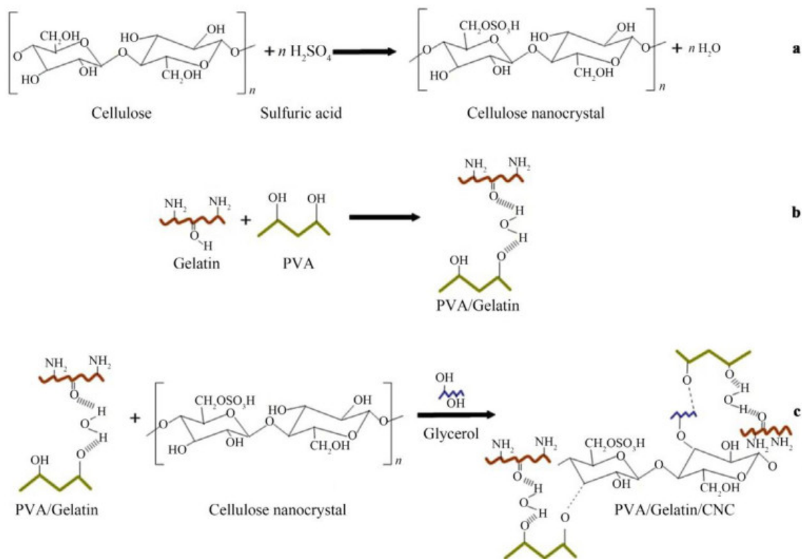
(a) Synthesis of CNC; (b) blending of PVA and gelatin; (c) fabrication of the films
