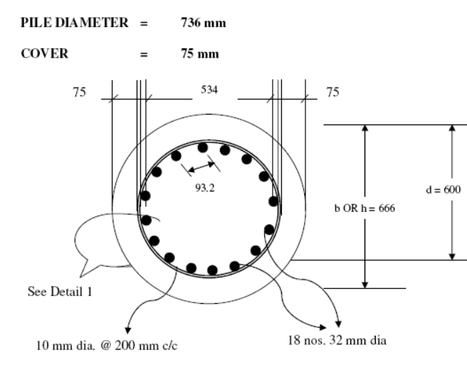
Sketch No. 1 (cross section of steel cage)
