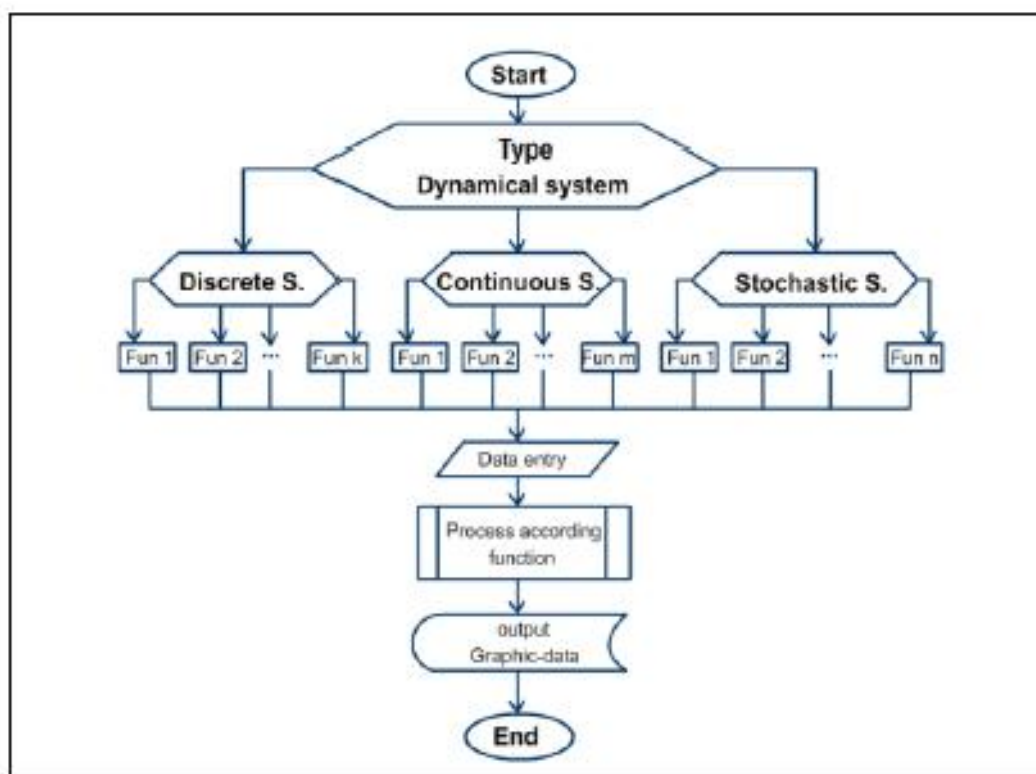
Figure 2. DSamala toolbox flowchart
