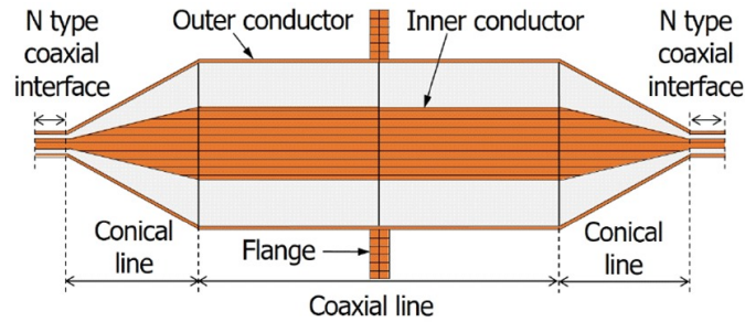
(a) ASTM D4935 단면도 (a) ASTM D4935 cross-section
